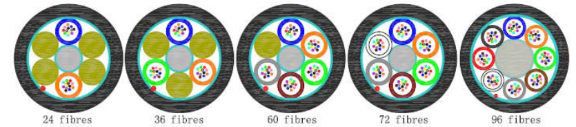
MiniCable 24~144 芯光纖微纜
